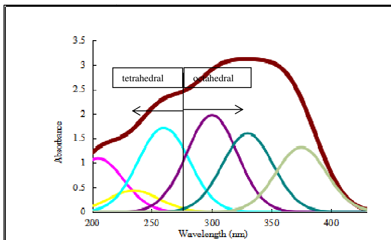
Fig. 2. Deconvolution of DR UV-Vis spectra of SiO 2 -TiO 2
