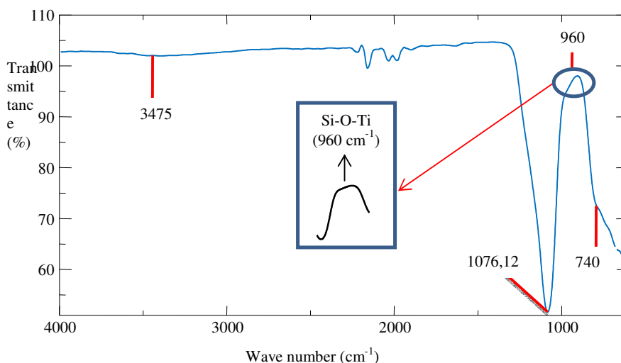
Fig. 1. FTIR spectrum of synthesized silica-titania catalyst.
