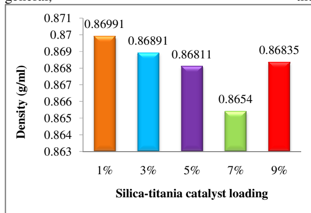
Fig. 3. The density of biodiesel from palm oil.
