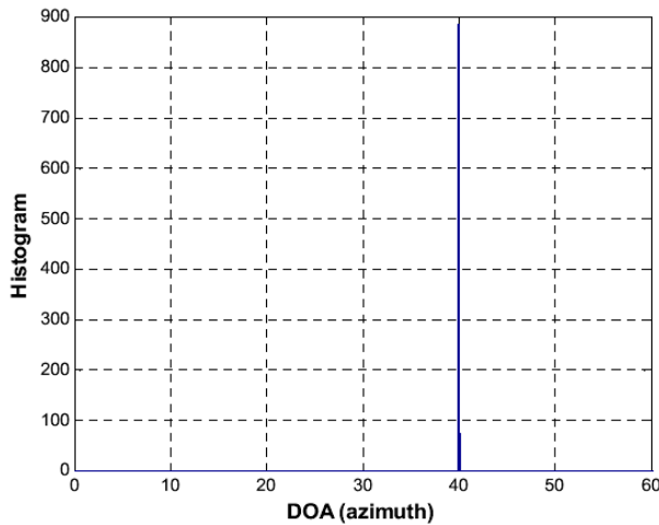
Fig. 2 PM Histogram for DOA (azimuth) estimation using parallel array configuration
