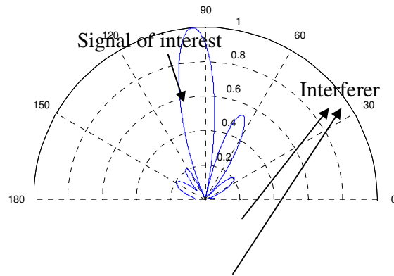
Fig. 3. Null steering beamformer
