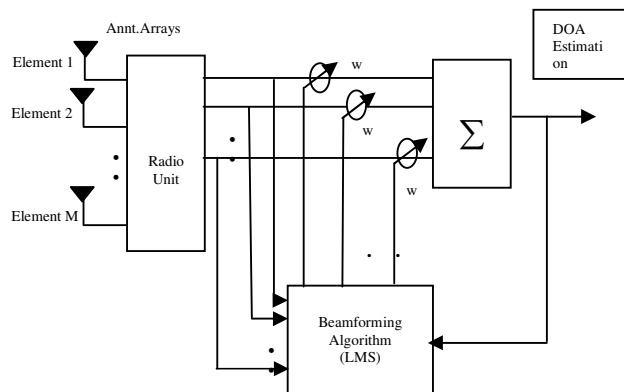
Fig. 1 Proposed Model for Propagator method for DOA estimation and beamforming
