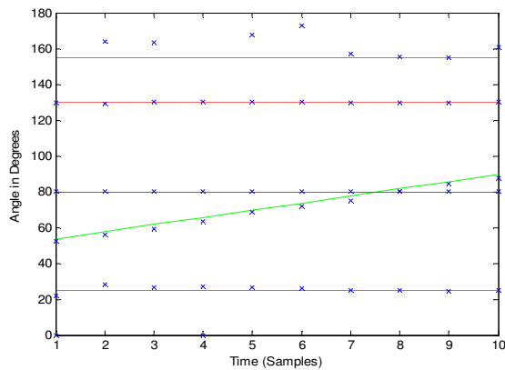
Fig. 2 Estimated Directions for Users using MUSIC Algorithm
