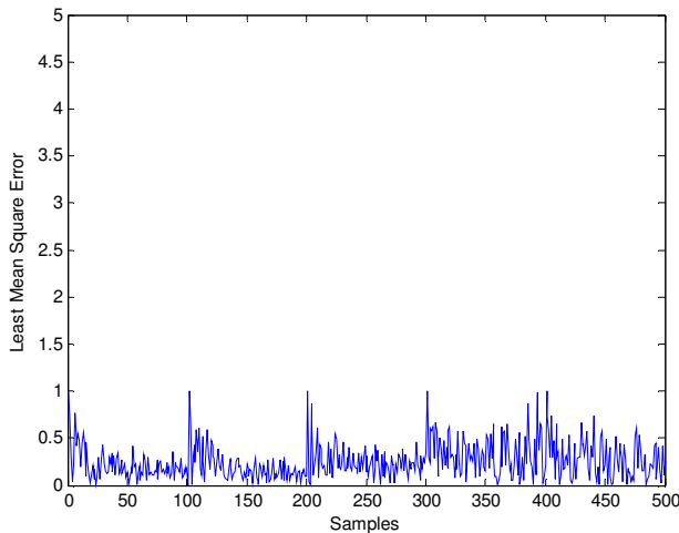
Fig. 6 LMS Error Plot for 500 Iteration
