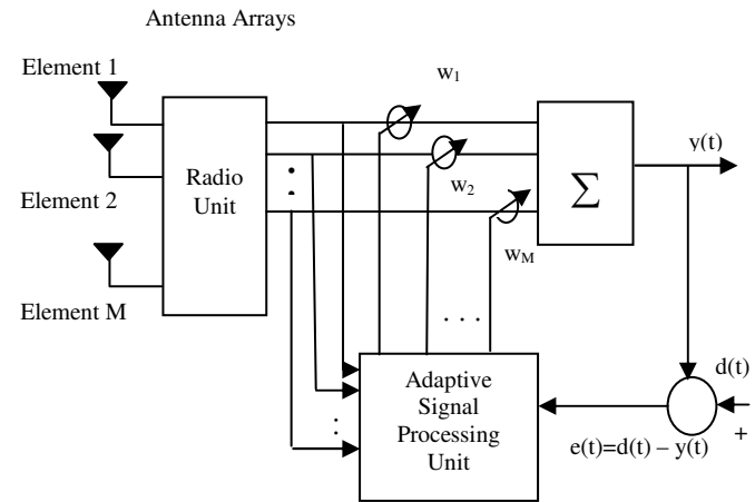
Fig.1 Smart Antenna System
