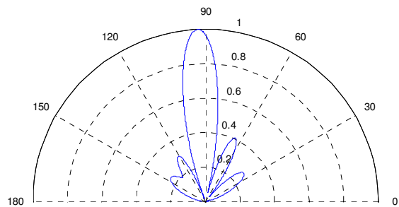
Fig. 4 Normalized Array Factor Plot for Dynamic Case
