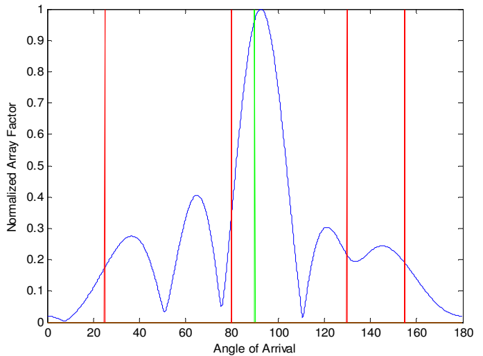
Fig. 4 Normalized Array Factor Plot for Dynamic Case
