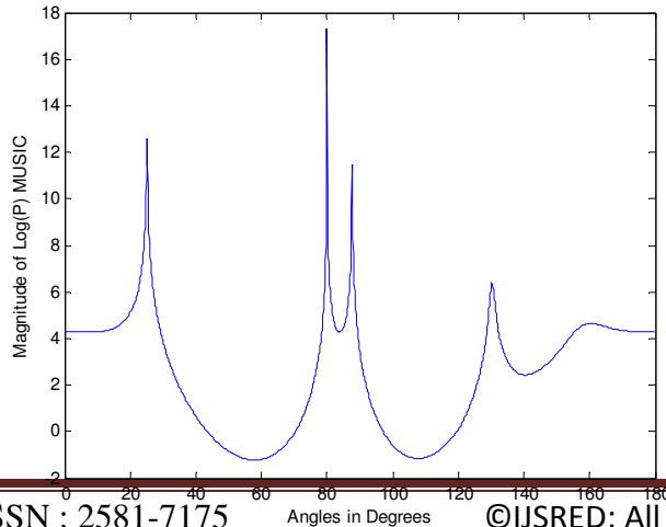
Fig. 2 Estimated Directions for Users using MUSIC Algorithm
