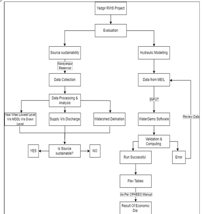
Fig 2: Process flow chart detailing the projects workflow
