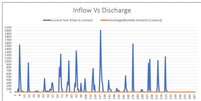
Fig 4: Inflow (Supply) Vs Discharge (Demand) Graph
