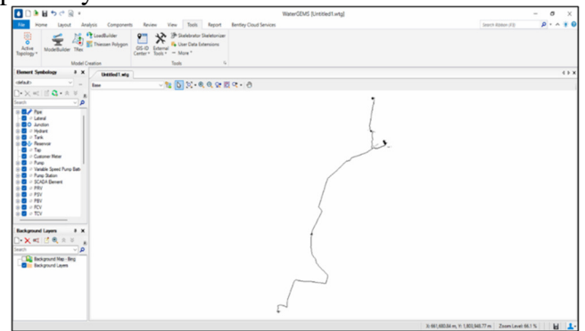
Fig 6: Hydraulic model of starting stretch of Yadgir- RWS Project in WaterGems interface
