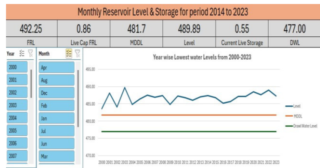
Fig 5: Annual lowest level of reservoir Vs Intake level for Project Vs MDDL
