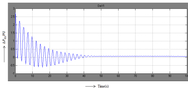
Change in power output of generator in area-1
