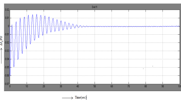
Deviation of frequency in area-1
