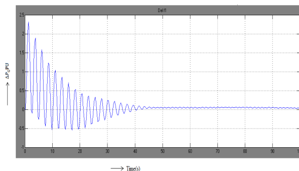
Change in power output of generator in area-2
