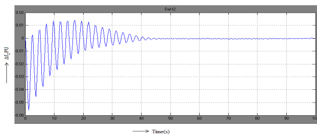
Deviation of frequency in area-2
