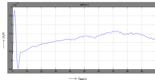
Waveform of deviation in tie-line power flow
