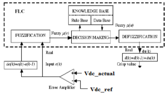
Fig. Block diagram of the Fuzzy Logic Controller (FLC) for Proposed Converter
