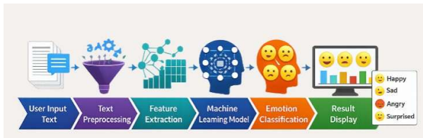
Fig. 1. System Workflow
